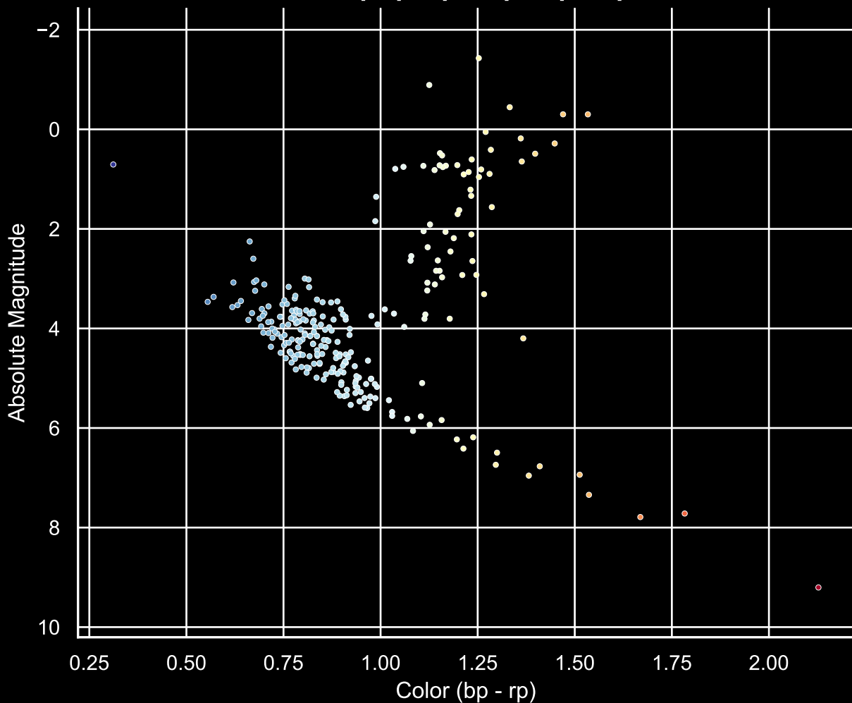
GALAH Hertzprung-Russel Diagram Field [104] Ra [321.42] Dec [-19.58]
