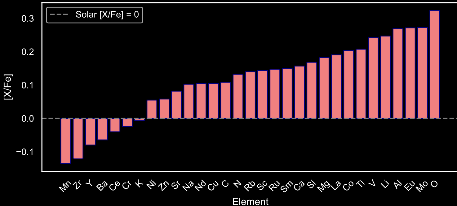
Abundance Pattern for GALAH Red Giants: Star Field [104] (N=55)
