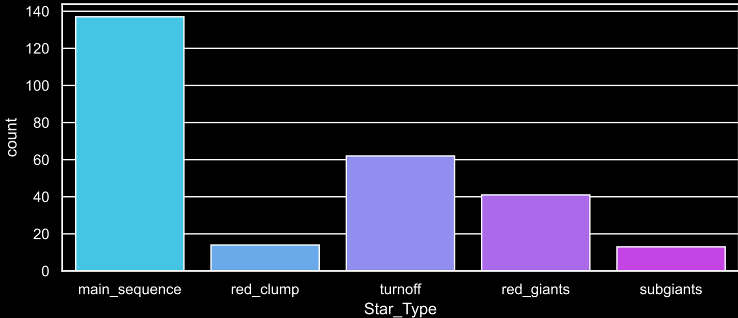
Field [104] Count plot of Star Type
