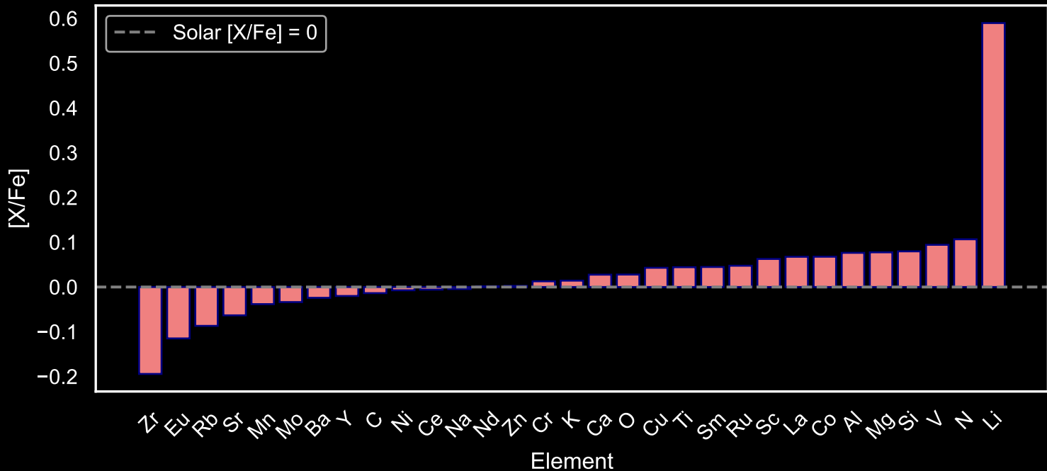
Abundance Pattern for GALAH Main Sequence Stars: Star Field [104] (N=137)
